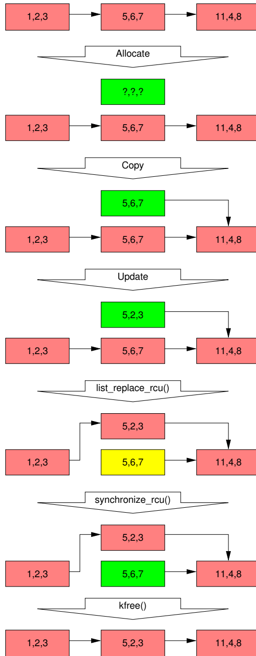
Figure 9.19: RCU Replacement in Linked List
